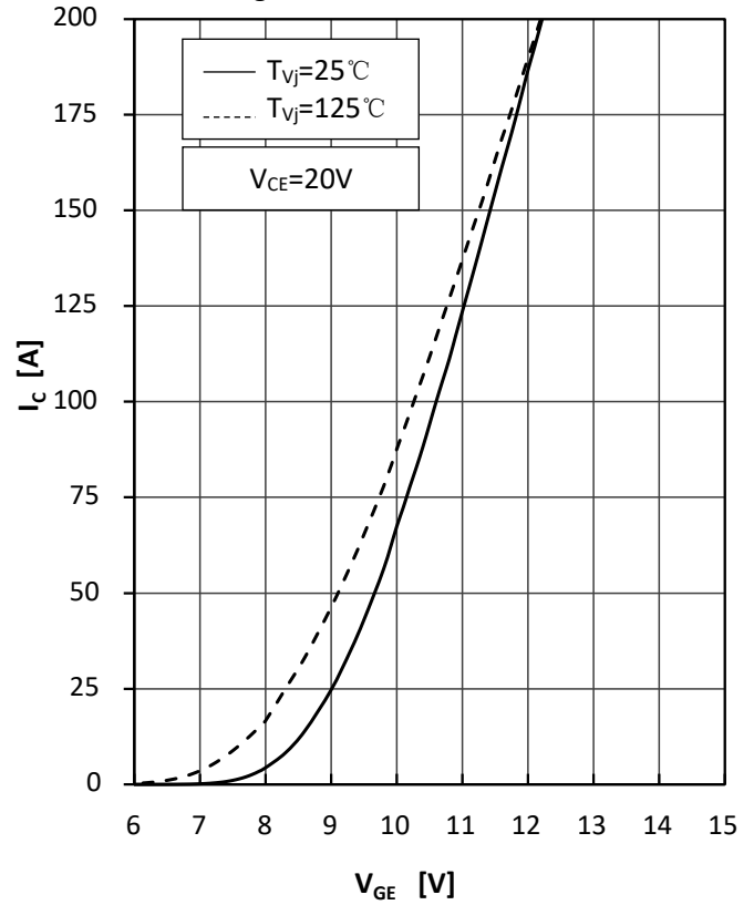
Fig2.IGBT Transfer Characteristics
