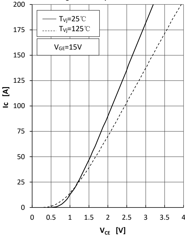
Fig1.IGBT Output Characteristics
