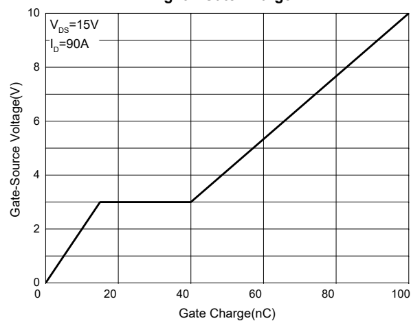
Fig. 6 - Gate Charge
