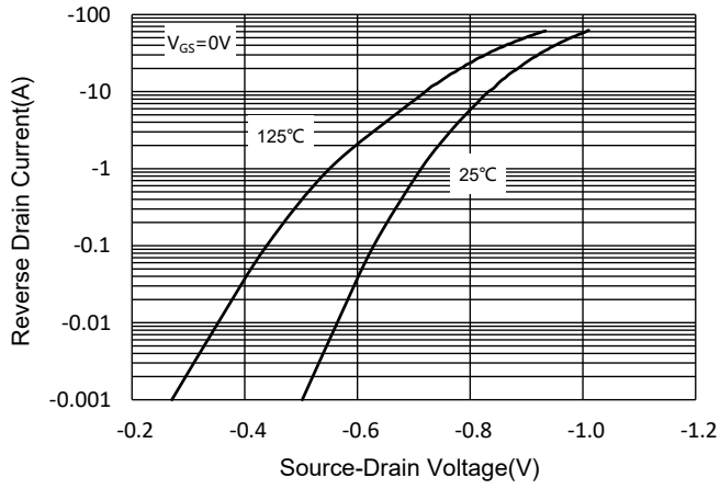
Fig.9 IS-VSD
