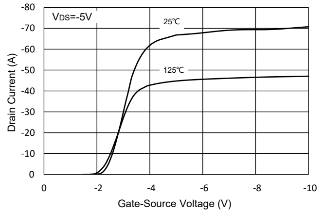
Fig.2 Transfer Characteristic
