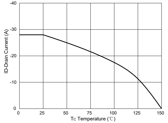
Fig.10 Drain Current
