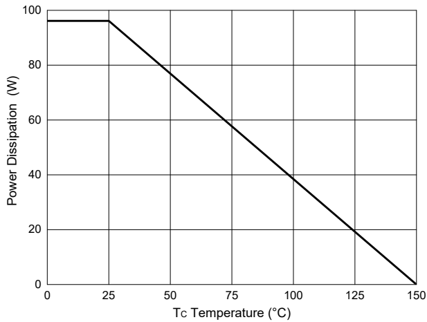
Fig.11 Power Dissipation
