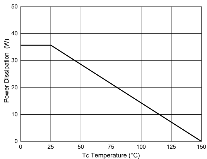
Fig.11-PD Dissipation
