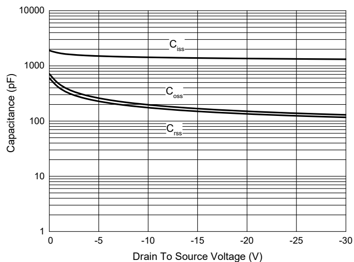
Fig. 5 - Capacitance Characteristics
