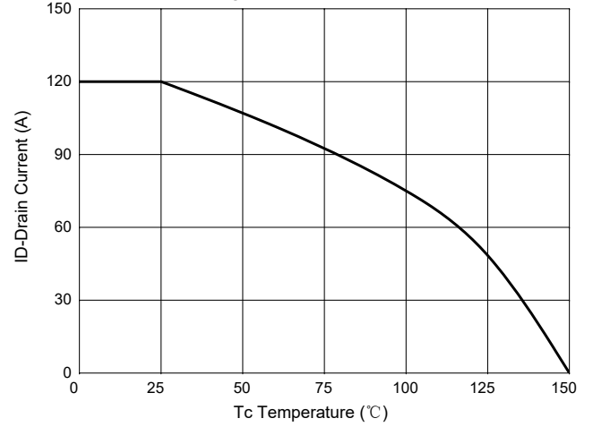
Fig. 10 - Drain Current
