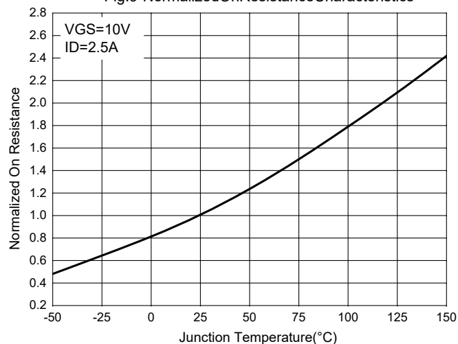
Fig.9-NormalizedOnResistanceCharacteristics
