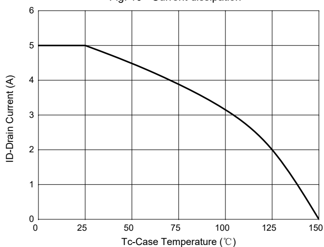
Fig. 10 - Current dissipation
