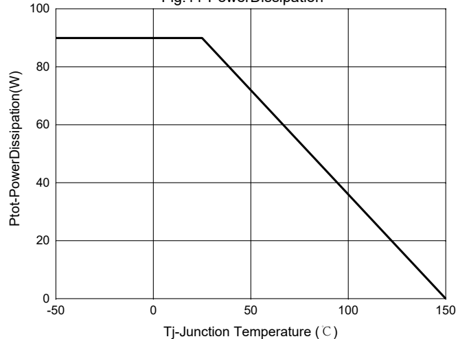
Fig.11-PowerDissipation
