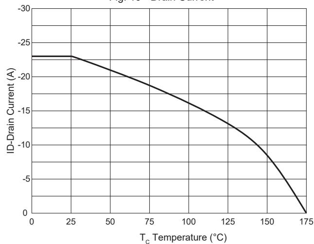
Fig. 10 - Drain Current
