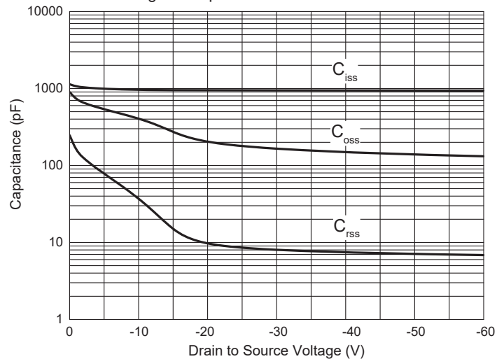
Fig. 5 - Capacitance Characteristics
