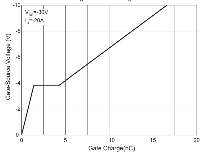
Fig. 6 - Gate Charge
