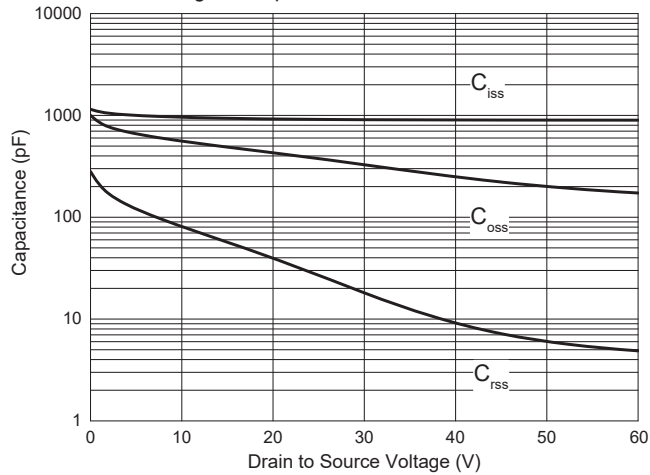
Fig. 5 - Capacitance Characteristics
