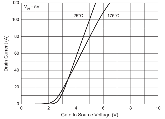
Fig. 2 - Transfer Characteristics
