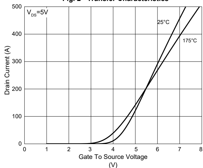
Fig. 2 - Transfer Characteristics
