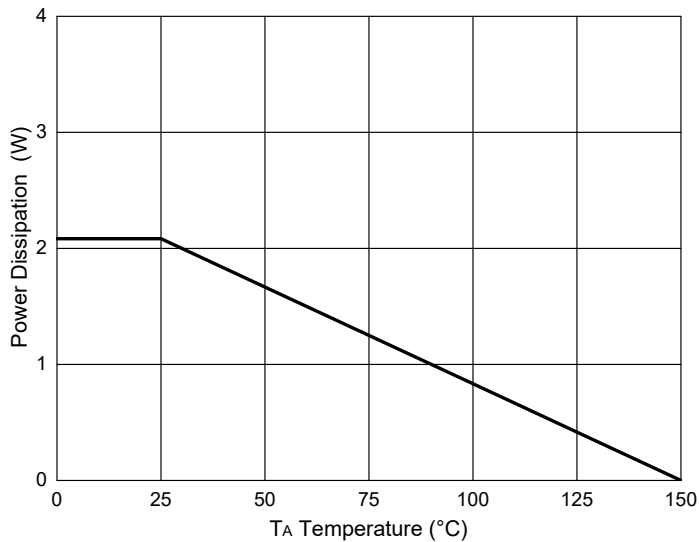
Fig.11-PD Dissipation
