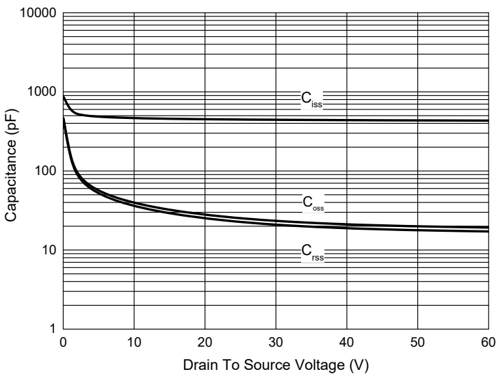
Fig. 5 - Capacitance Characteristics
