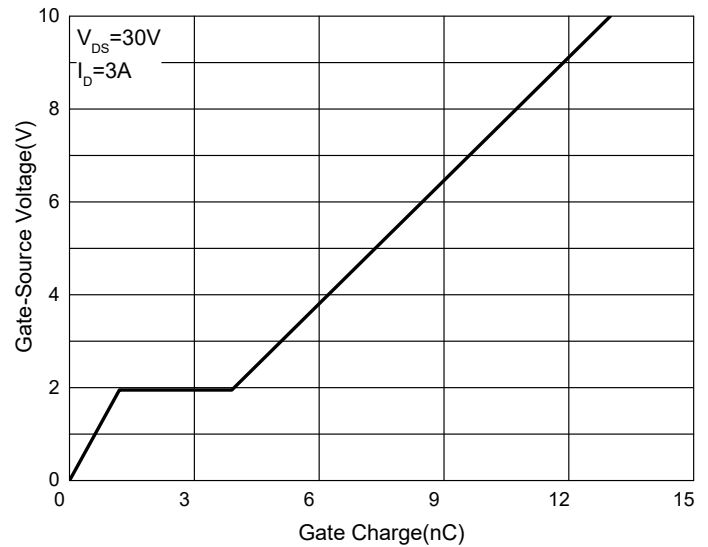
Fig. 6 - Gate Charge
