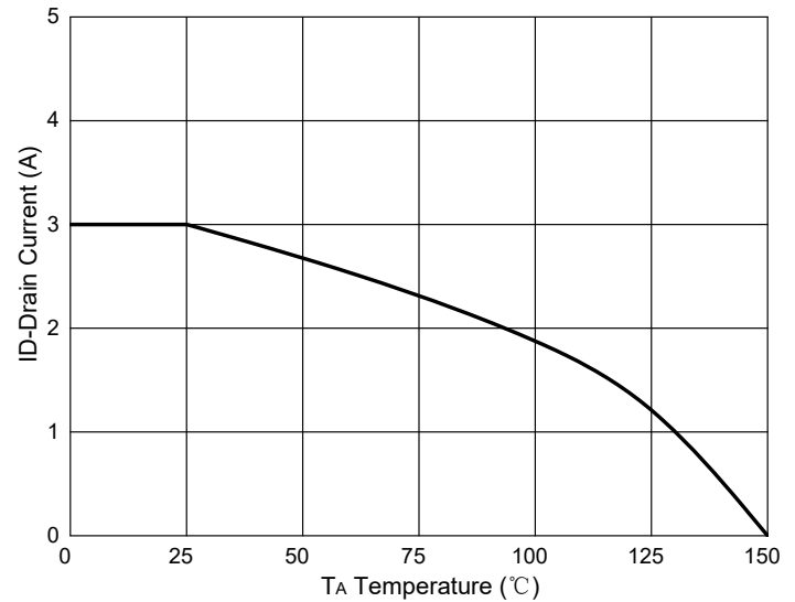
Fig. 10 - Drain Current
