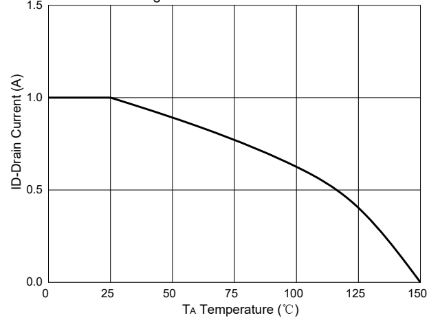
Fig. 10 - Drain Current
