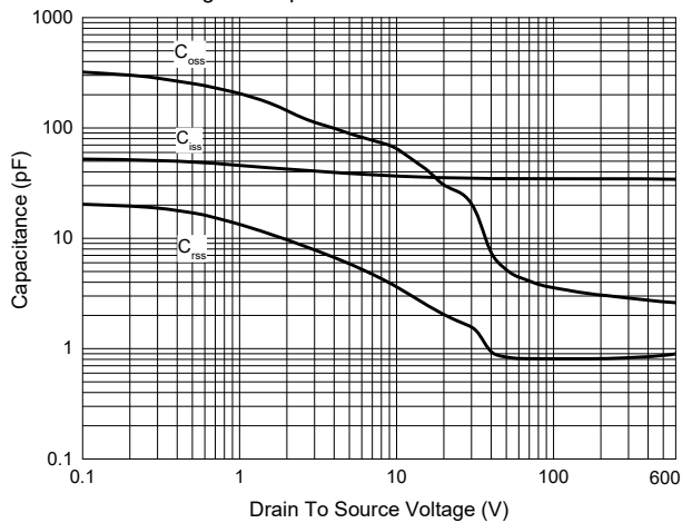
Fig. 5 - Capacitance Characteristics
