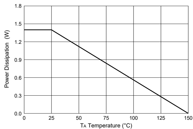
Fig.11 - PD Dissipation
