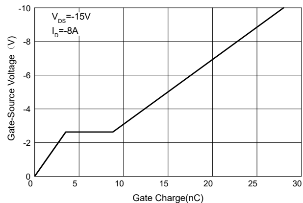
Fig.6 - Gate Charge
