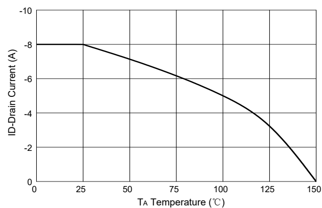
Fig.10 - Drain Current
