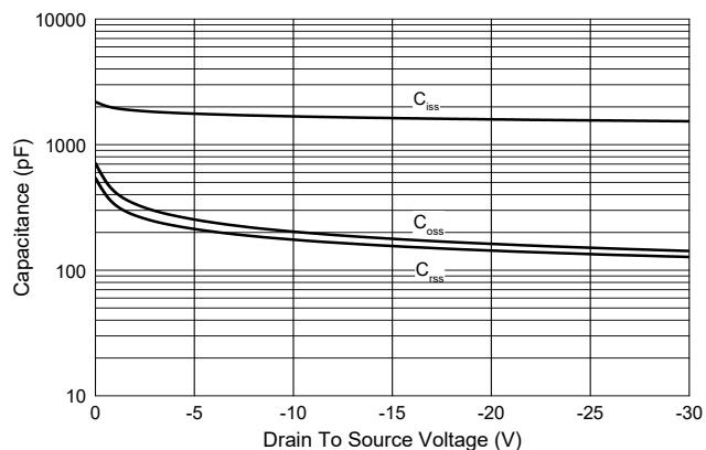
Fig.5 - Capacitance Characteristics
