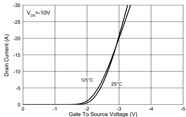
Fig.2 - Transfer Characteristic
