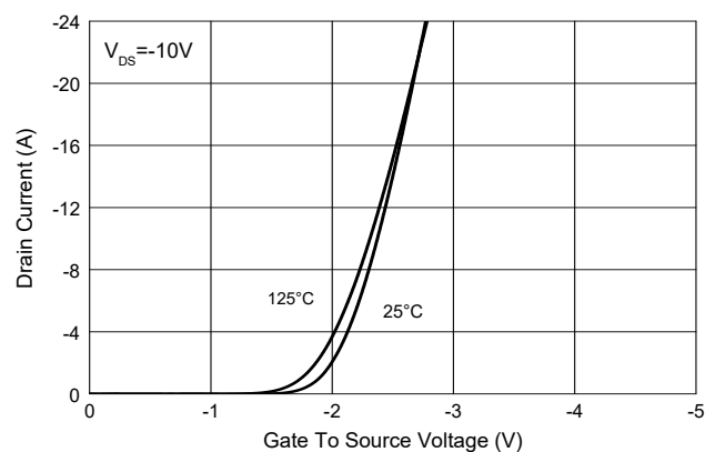
Fig.2 - Transfer Characteristic
