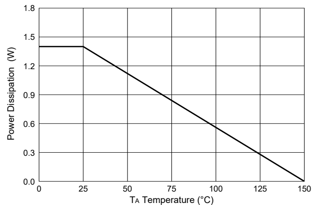
Fig.11 - PD Dissipation
