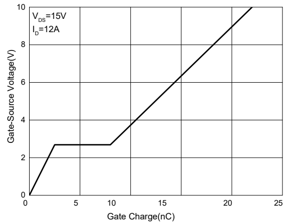
Fig.6 - Gate Charge
