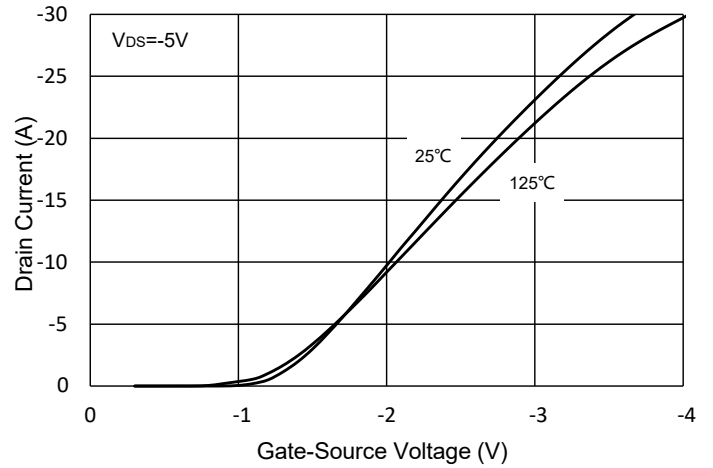
Fig.2 Transfer Characteristic
