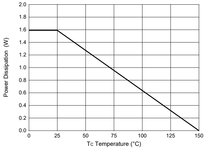
Fig.11-PD Dissipation
