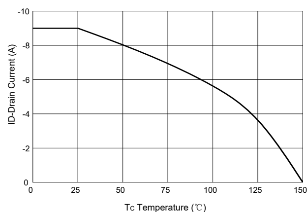
Fig. 10 - Drain Current
