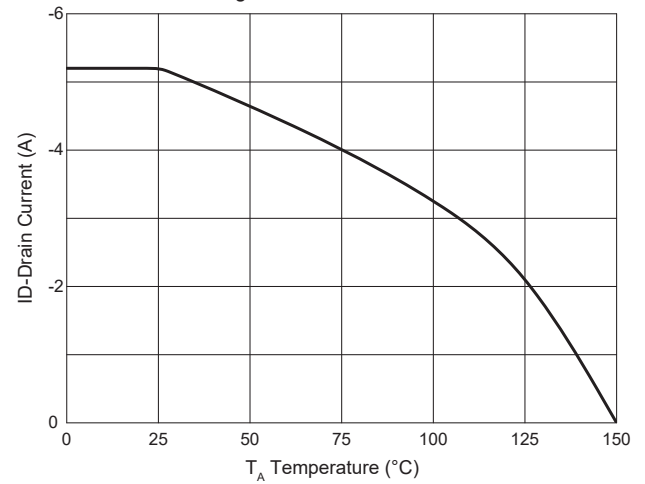
Fig. 10 - Drain Current
