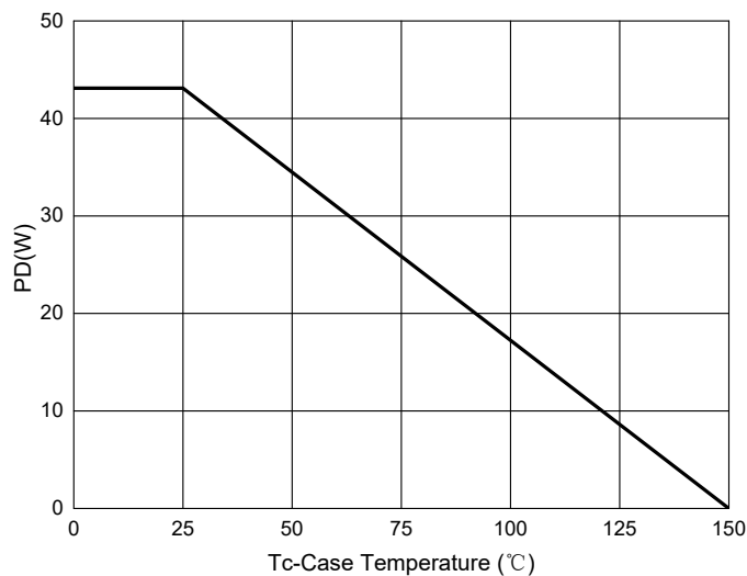
Fig. 11 - Power Dissipation
