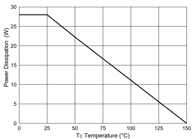
Fig.11-PD Dissipation
