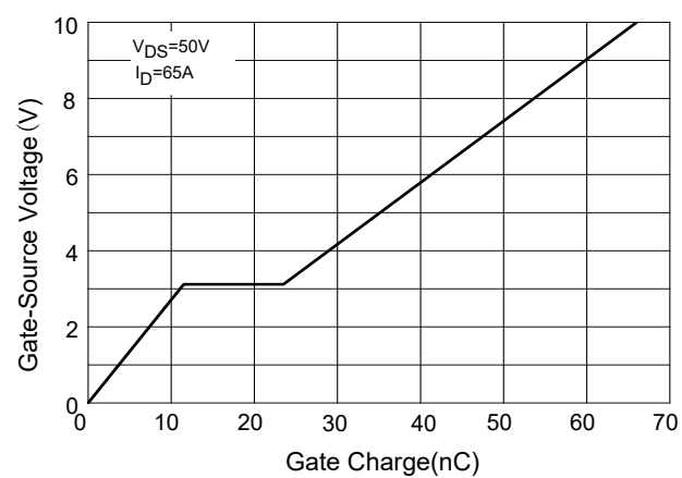
Fig.6 - Gate Charge
