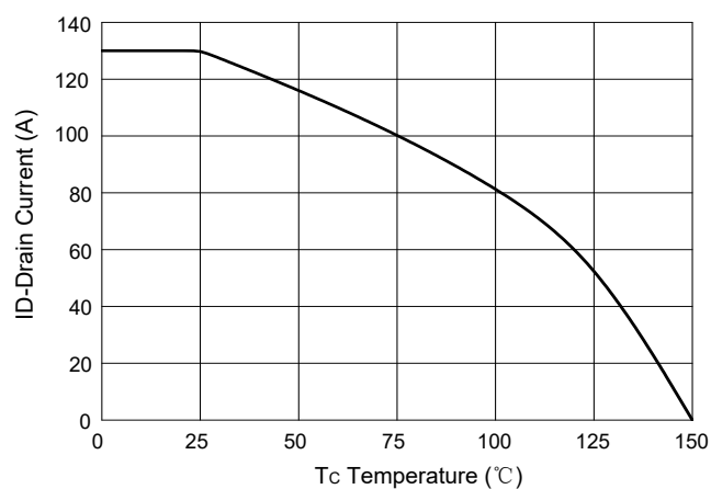
Fig.10 - Drain Current
