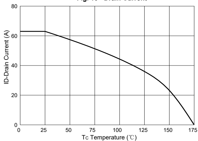
Fig. 10 - Drain Current
