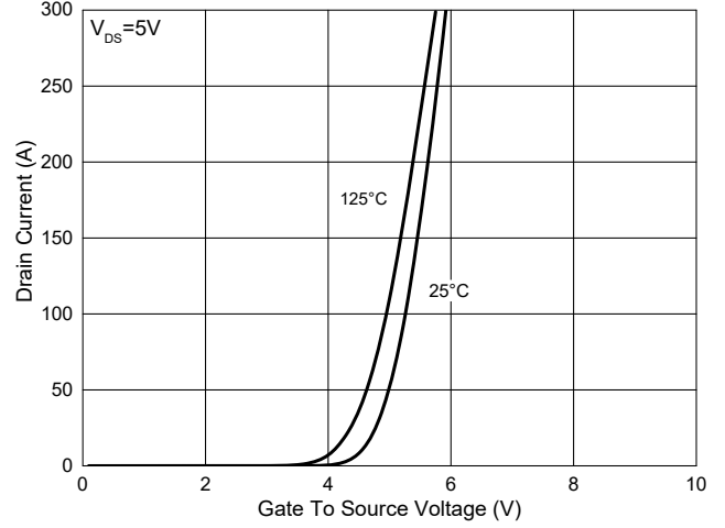
Fig. 2 - Transfer Characteristics
