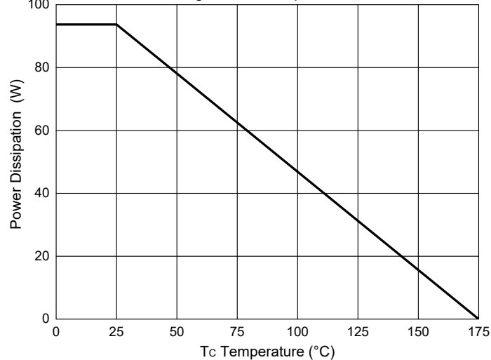
Fig.11-PD Dissipation
