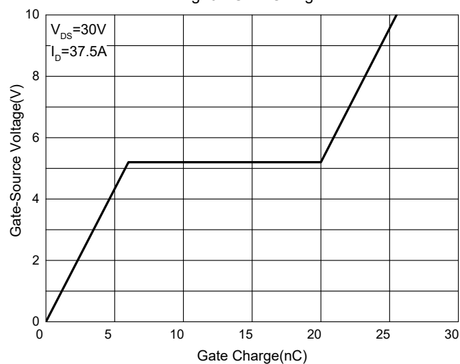
Fig. 6 - Gate Charge
