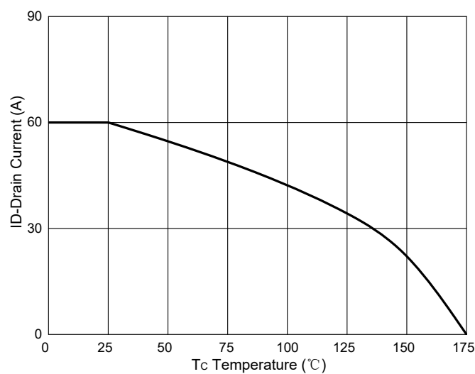
Fig. 10 - Drain Current
