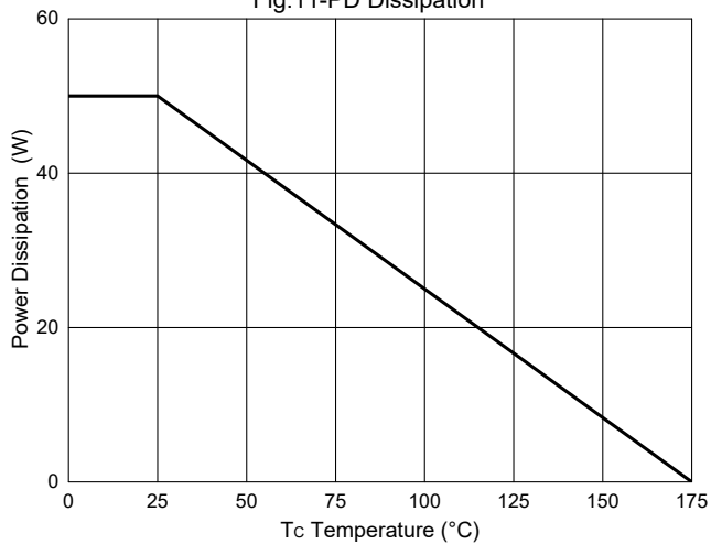
Fig.11-PD Dissipation
