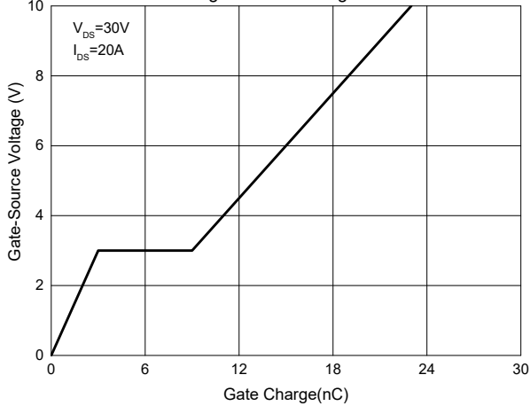
Fig. 5 - Gate Charge
