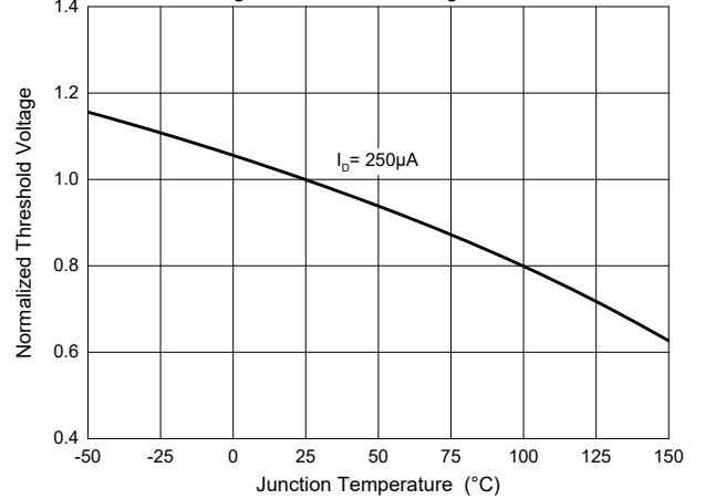
Fig. 6 - Threshold Voltage
