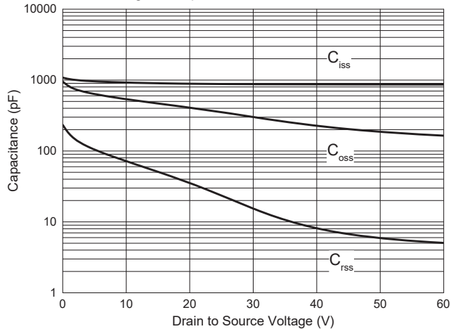
Fig. 5 - Capacitance Characteristics
