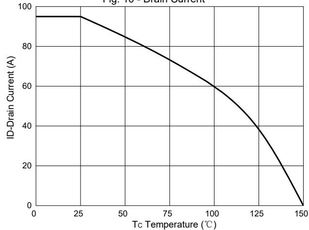
Fig. 10 - Drain Current
