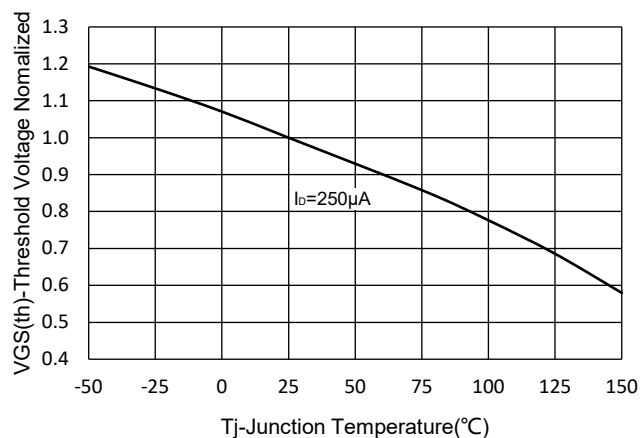
Fig.7-Normalized Threshold Voltage
