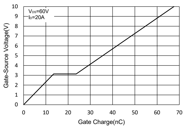
Fig.6 -Charge
