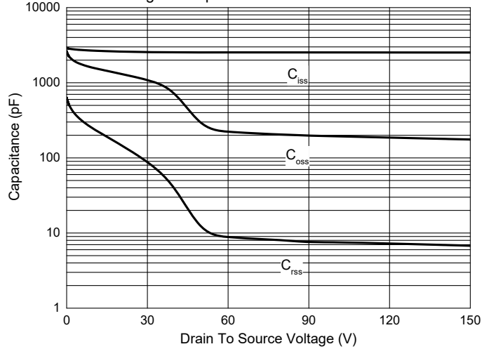
Fig. 5 - Capacitance Characteristics
