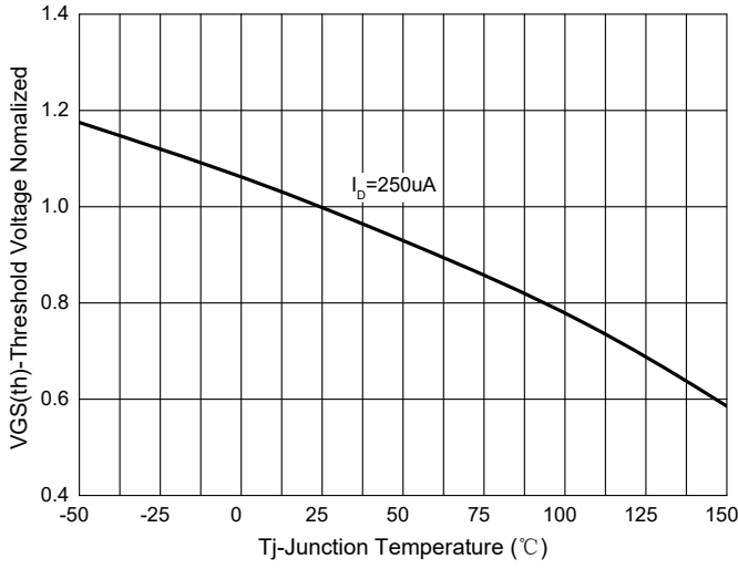
Fig. 7 - Normalized Threshold voltage
