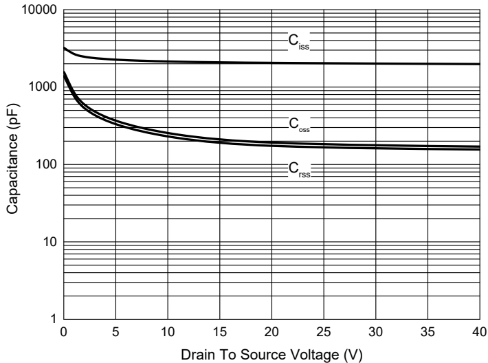
Fig. 5 - Capacitance Characteristics
