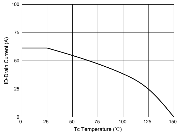
Fig. 10 - Current dissipation
