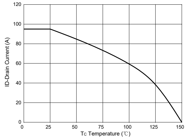
Fig. 10 - Drain Current
