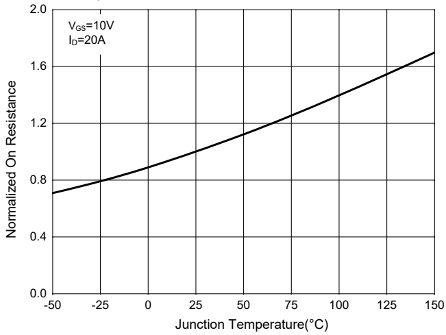
Fig.7-NormalizedOnResistanceCharacteristics
