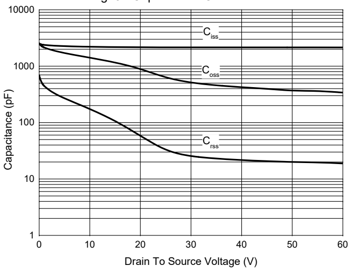
Fig. 5 - Capacitance Characteristics
