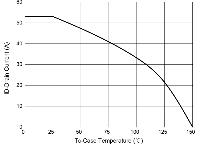
Fig. 10 - Current dissipation
