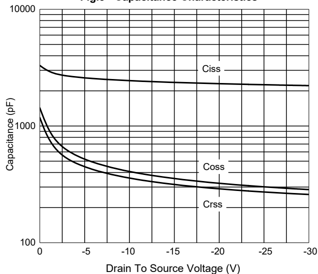
Fig.5 - Capacitance Characteristics
