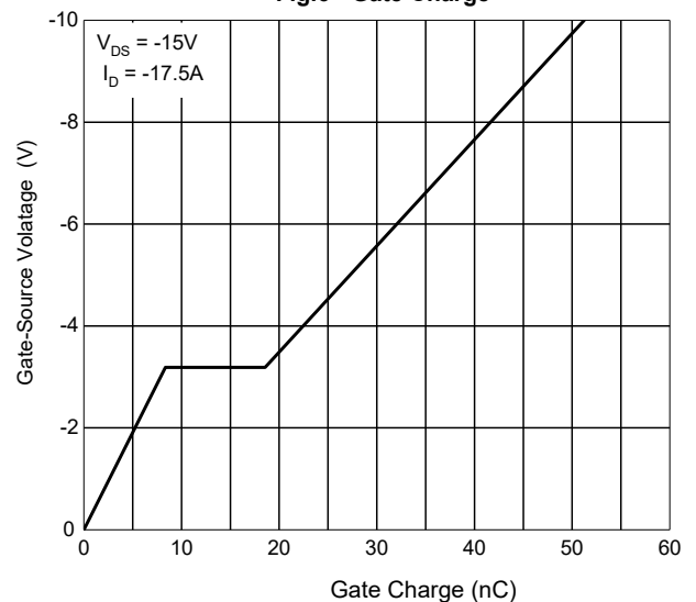
Fig.6 - Gate Charge
