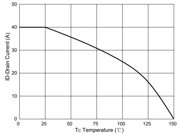
Fig.10 - Drain Current
