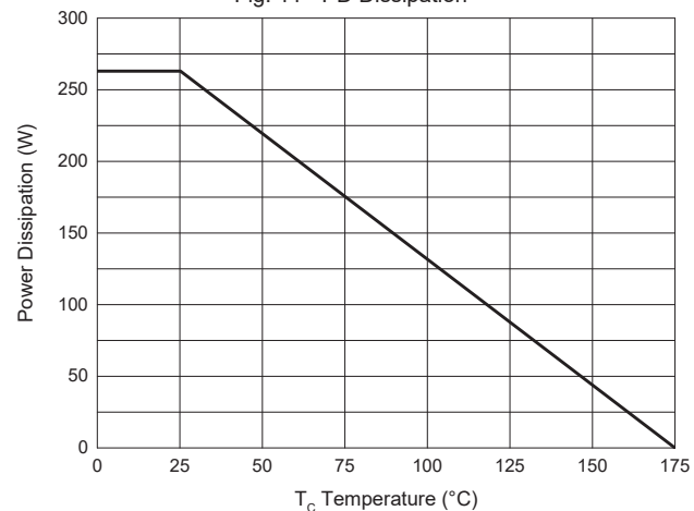
Fig. 11 - PD Dissipation
