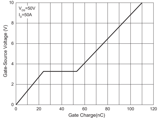
Fig. 6 - Gate Charge
