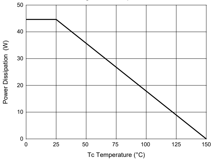
Fig.11-PD-dissipation
