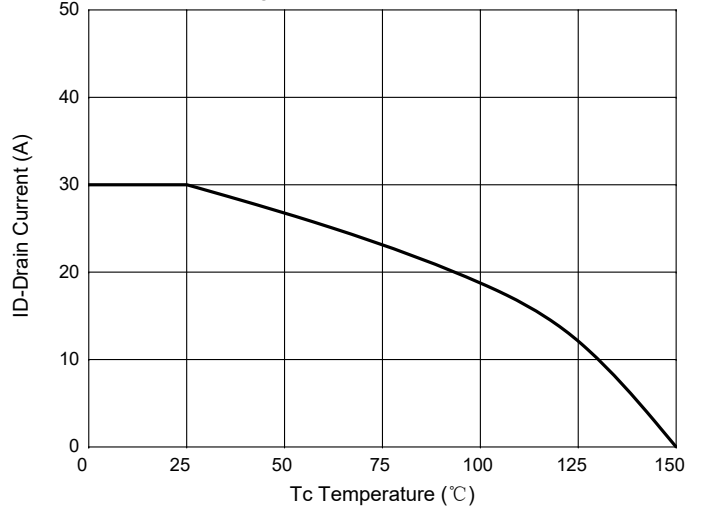
Fig. 10 - Current dissipation
