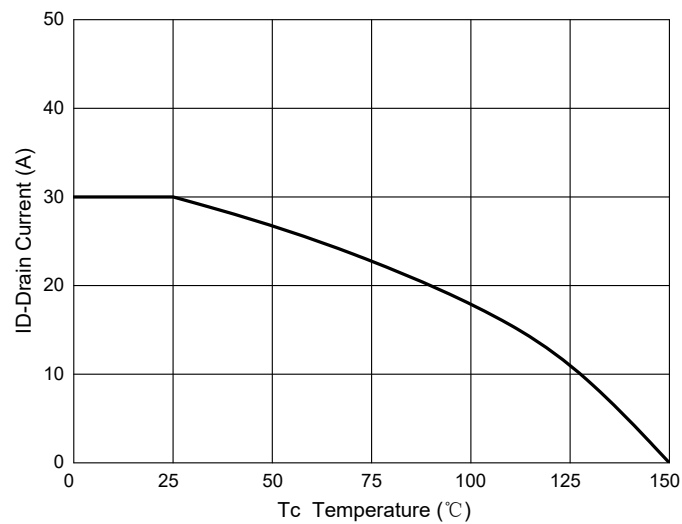
Fig. 10 - Drain Current
