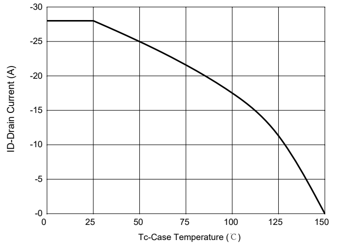
Fig. 10 - Current dissipation
