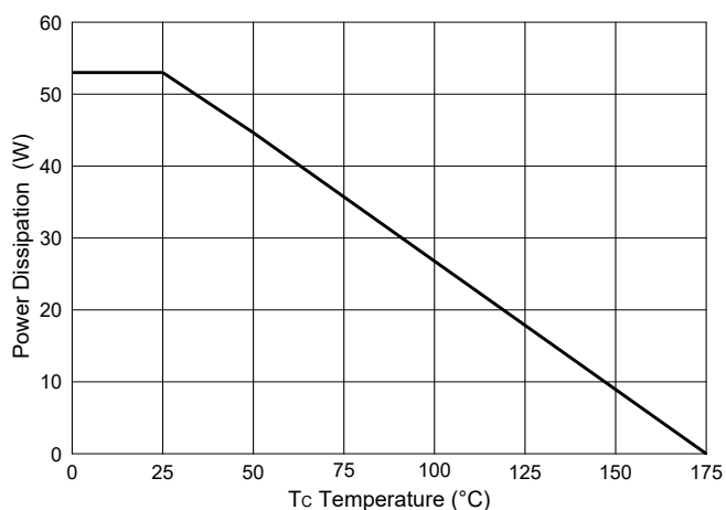
Fig.11-PD Dissipation
