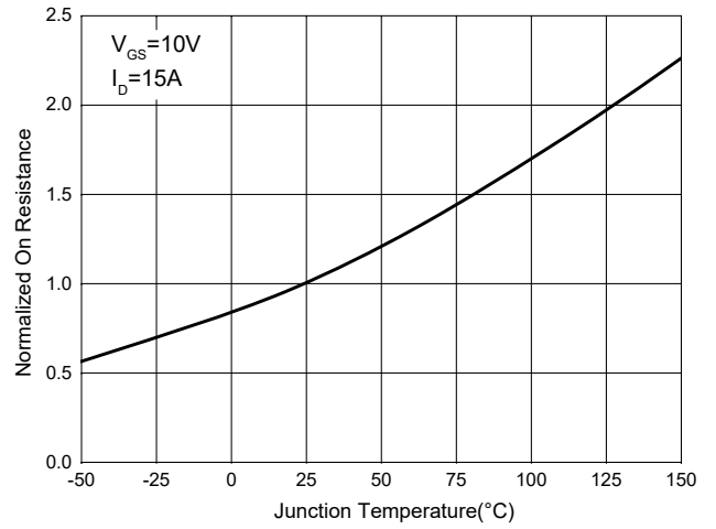
Fig.9-Normalized On Resistance Characteristics
