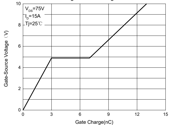
Fig. 6 - GateCharge
