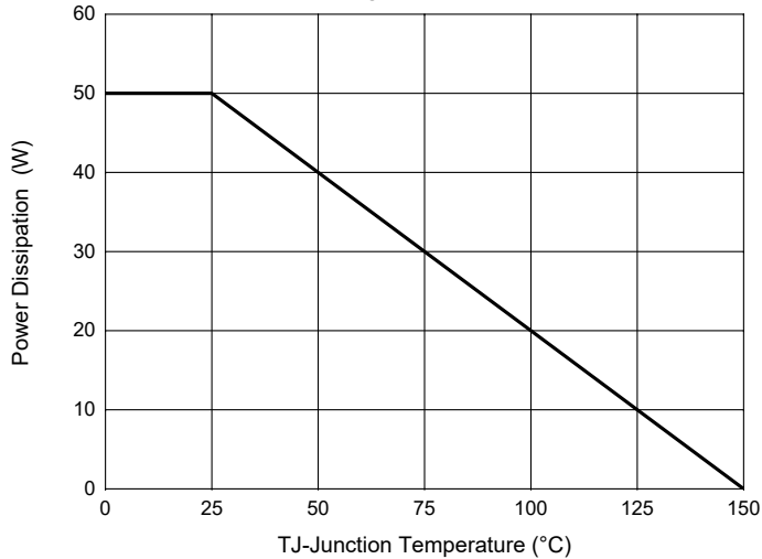
Fig.11-PD-TJ
