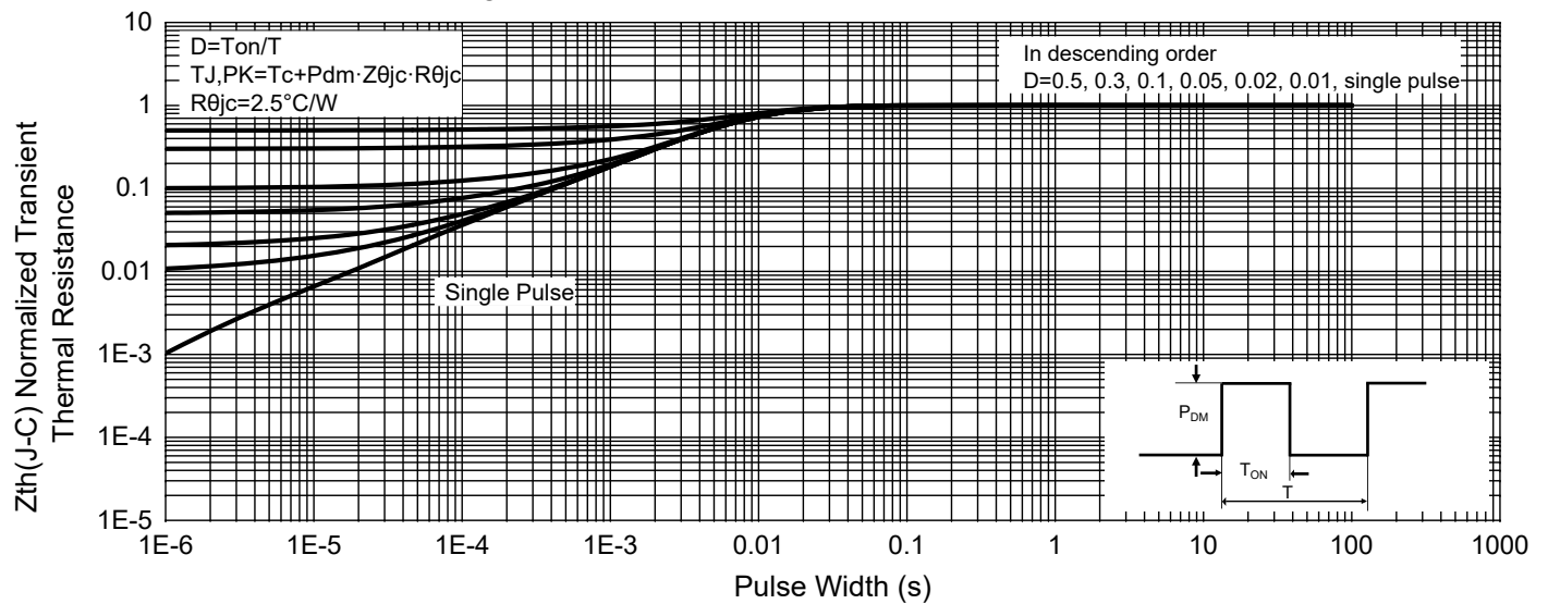
Fig. 13 - Normalized Transient Thermal Impedance
