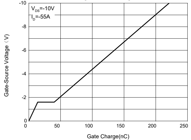
Fig. 6 - Gate Charge
