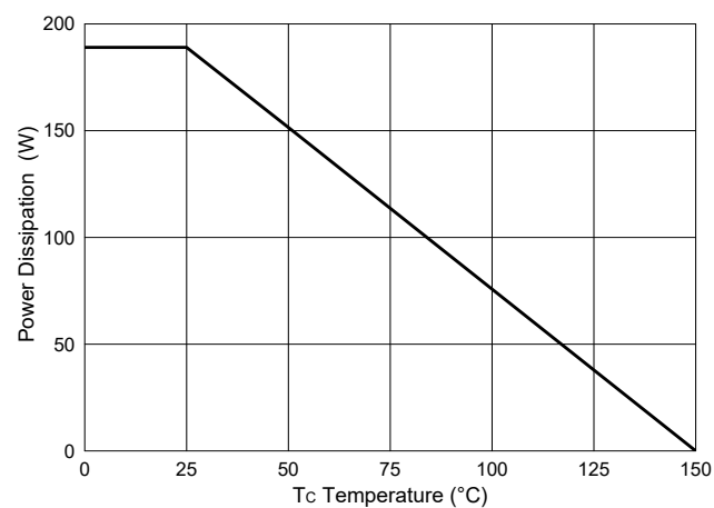
Fig.11-PD Dissipation
