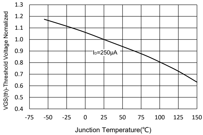
Fig.7 Threshold Voltage
