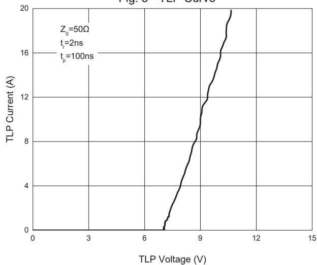
Fig. 5 - TLP Curve
