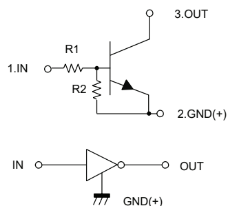
Internal Structure
