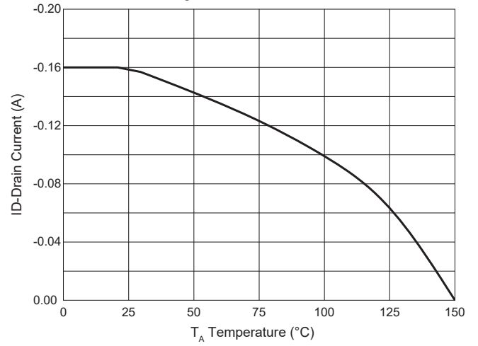
Fig. 10 - Drain Current
