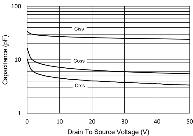
Fig.5 - Capacitance Characteristics
