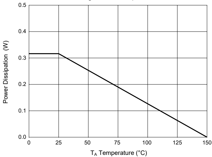
Fig.11-PD Dissipation
