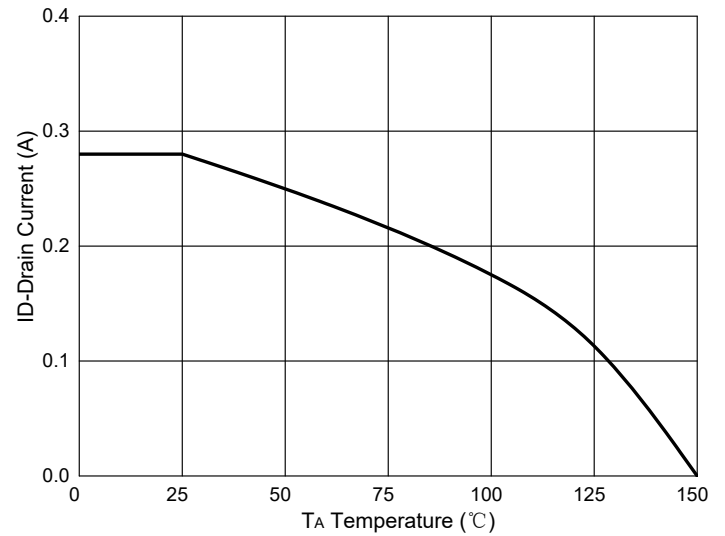
Fig. 10 - Drain Current
