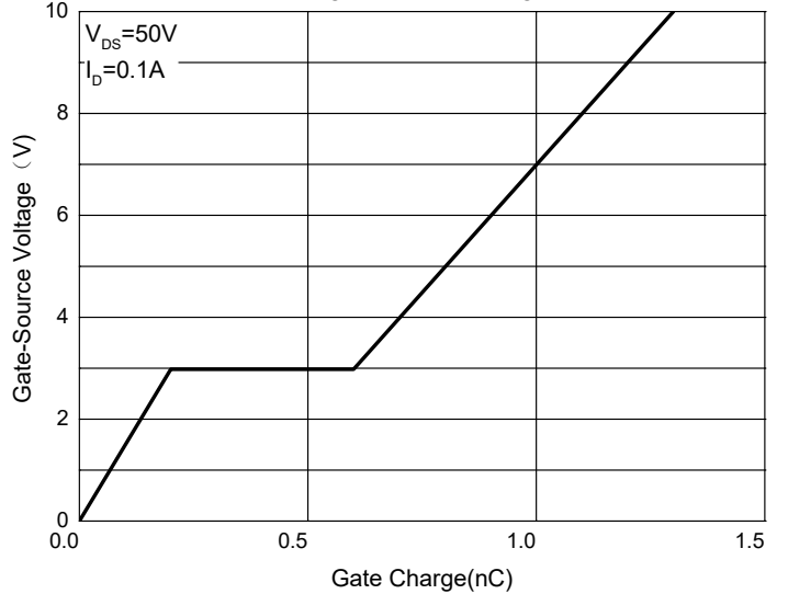
Fig. 6 - Gate Charge
